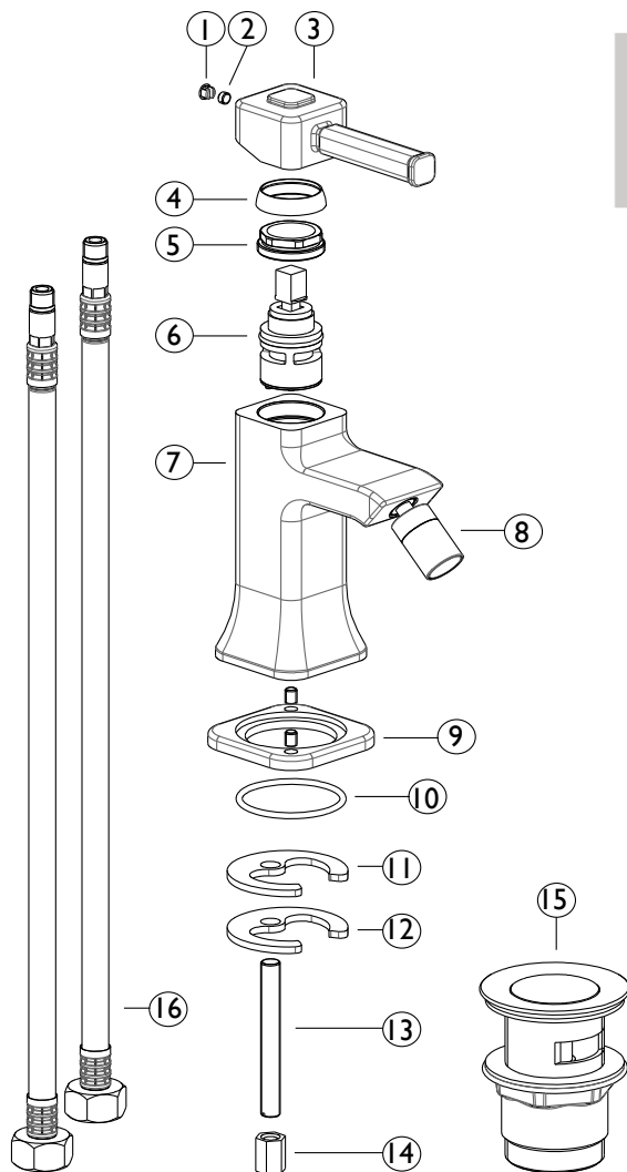
Illustration of bidet mixer only
