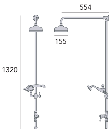
Fixed Riser Kit with Diverter to Head and Handset
