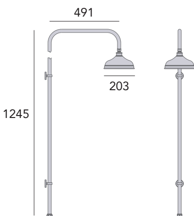
Deluxe Fixed Riser Kit with Head
