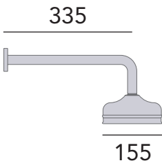
Large 6" shower head.
